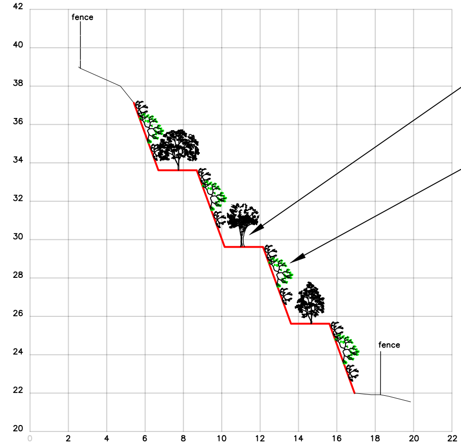
REPLANTING ACROSS STEPPED SLOPE
