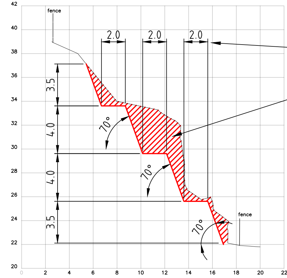
TYPICAL PROFILE AND DIMENSIONS OF STEPPED ROCKCUT
